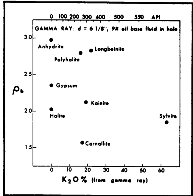
Fig. 18-3 — Crossplot of bulk density and apparent K_2O content (from Fig. 18-4) identifies potash minerals. (Courtesy SPWLA, Ref. 9)
