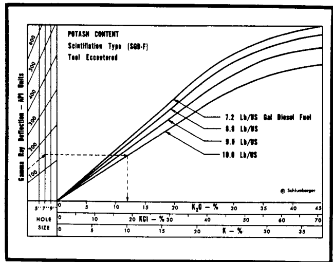
Fig. 18-4 — Empirical chart relating Gamma Ray Log deflection and apparent potassium content. (Courtesy SPWLA, Ref. 9)
