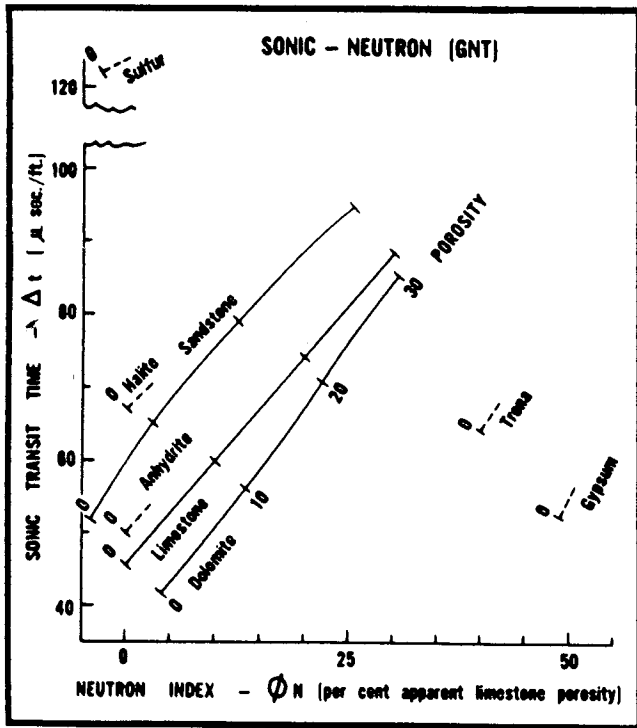
Fig. 18-2 — Sonic-Neutron crossplot for mineral identification. (Courtesy SPWLA, Ref. 9)
