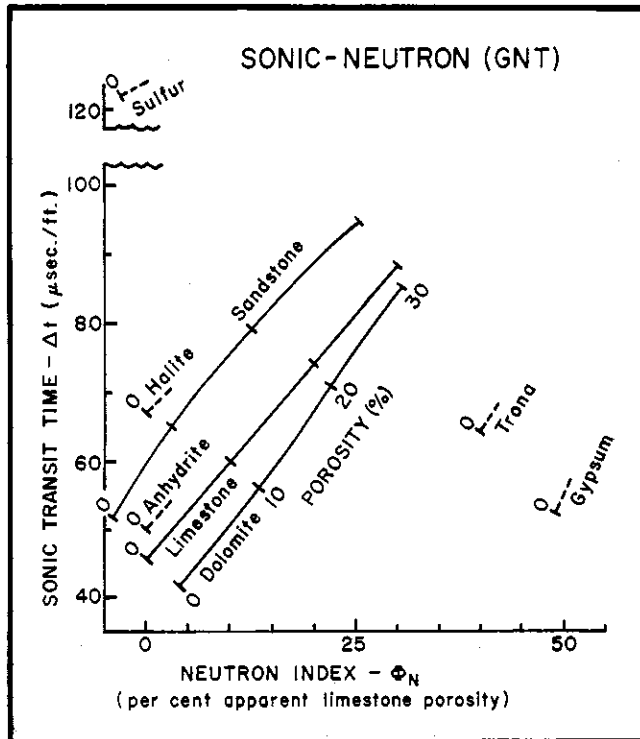
Fig. 18-2 — Sonic-Neutron crossplot for mineral identification. (Courtesy SPWLA, Ref. 10)
