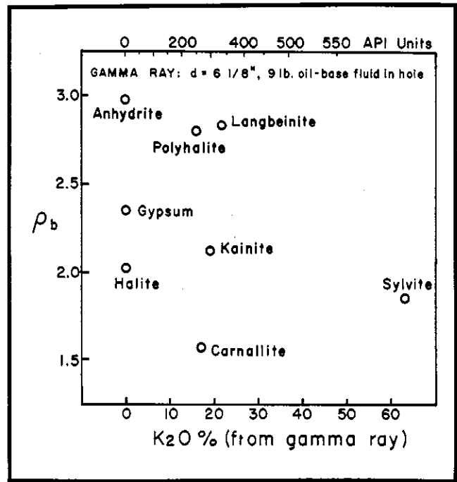
Fig. 18-3 — Crossplot of bulk density and apparent K_2O content (from Fig. 18-4) identifies potash minerals. (Courtesy SPWLA, Ref. 10)
