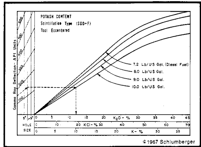
Fig. 18-4 — Empirical chart relating Gamma Ray Log deflection and apparent potassium content. (Courtesy SPWLA, Ref. 10)
